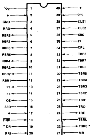
FIGURE 5. Pin Configuration
