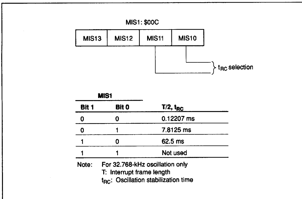
Figure 18 Miscellaneous Register 1
