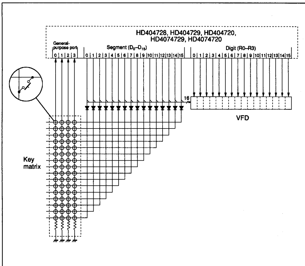
Figure 43 Example of VFD Connection
