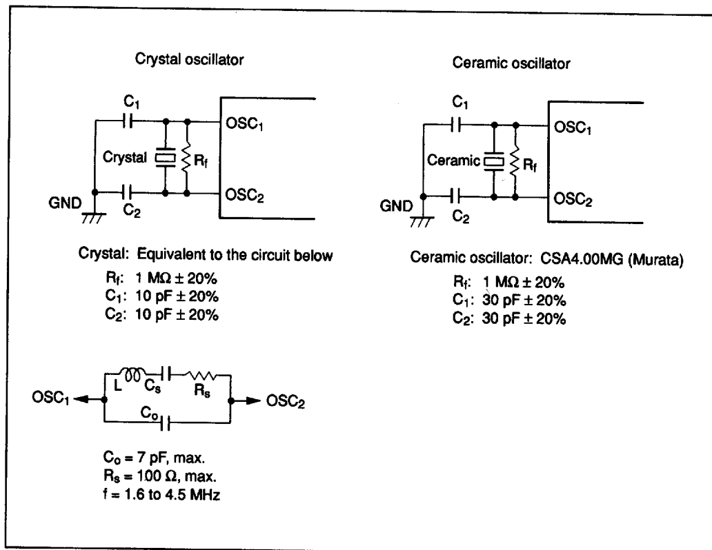
Figure 56 Oscillation Circuits (1)
