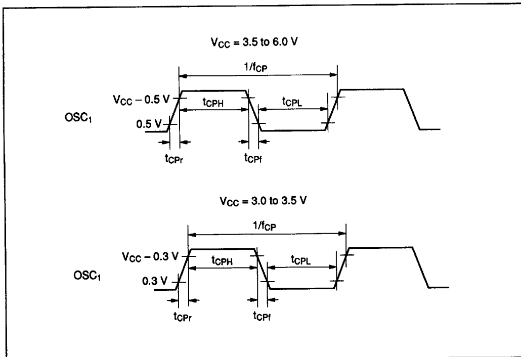
Figure 58 Oscillator Timing
