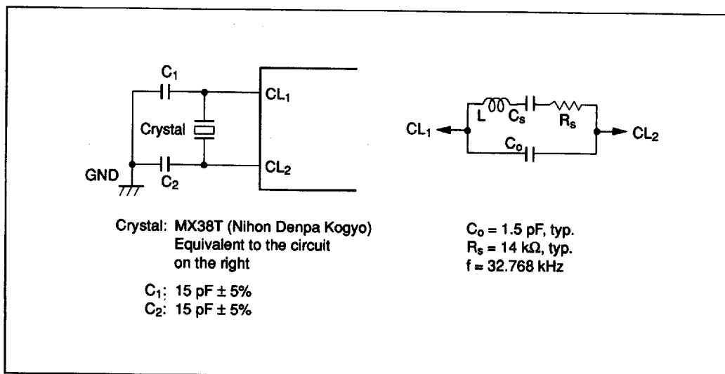
Figure 57 Oscillation Circuits (2)
