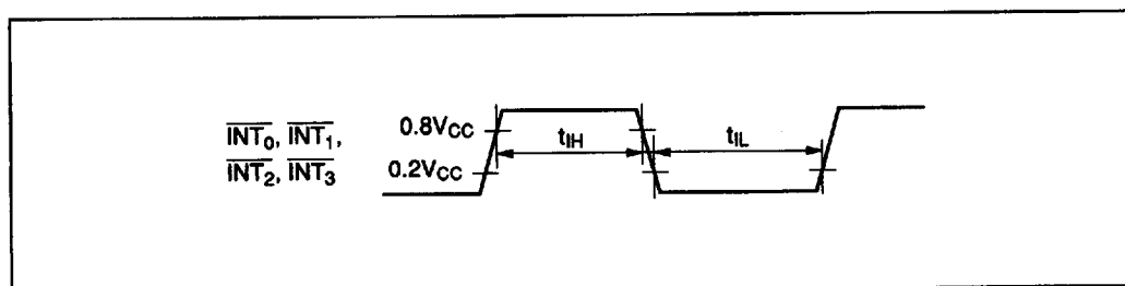
Figure 59 Interrupt Timing
