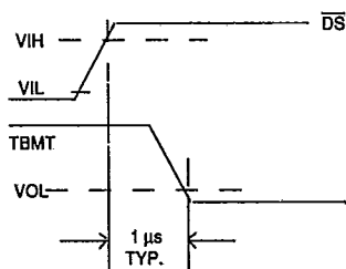
FIG. 14 TBMT TURN - OFF
