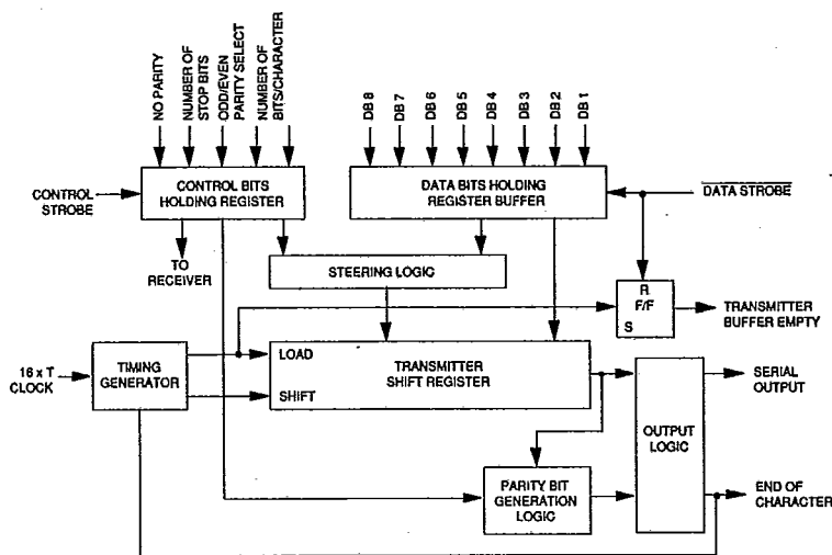
FIG. 24 TRANSMITTER BLOCK DIAGRAM
