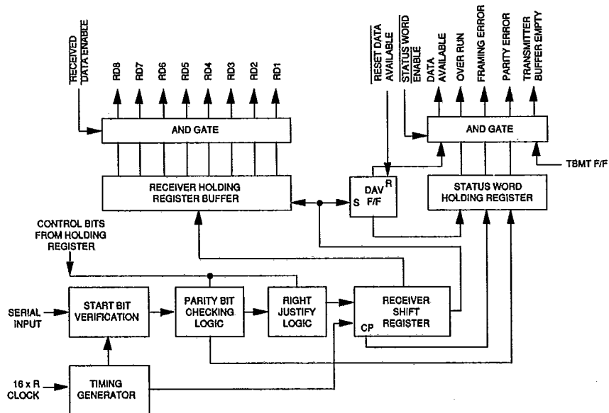
FIG. 25 RECEIVER BLOCK DIAGRAM
