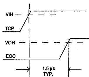
FIG. 13 EOC TURN - ON
