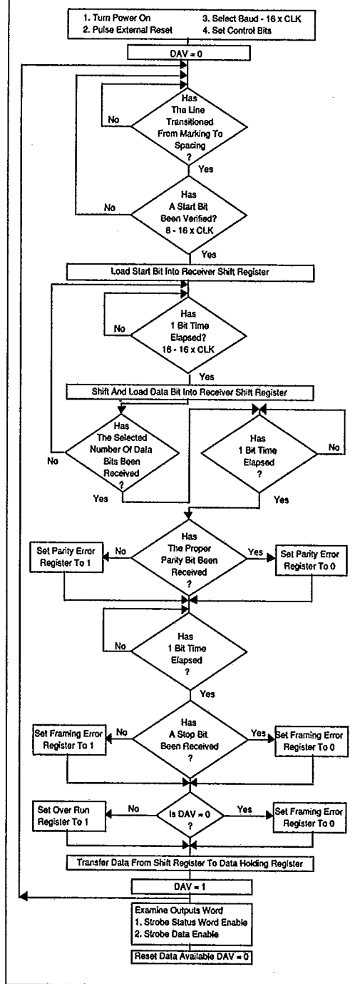
FIG. 23 RECEIVER OPERATION
