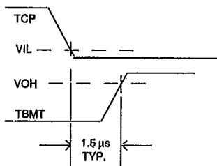
FIG. 16 TBMT TURN - ON
