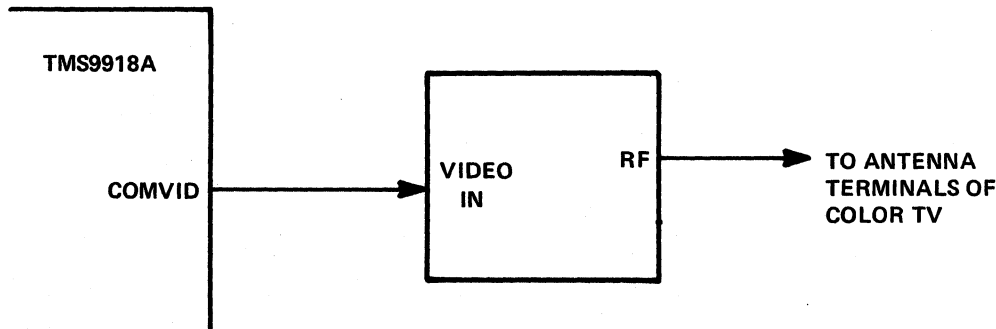
FIGURE 4-4 — RF MODULATOR CONNECTION
