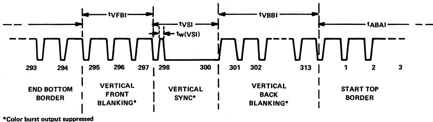
FIGURE 5-13 — TMS9929A VERTICAL TIMING
