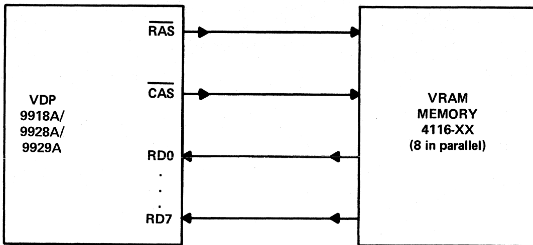
FIGURE B-1 — MEMORY CONFIGURATION SHOWING DELAY TIMES
