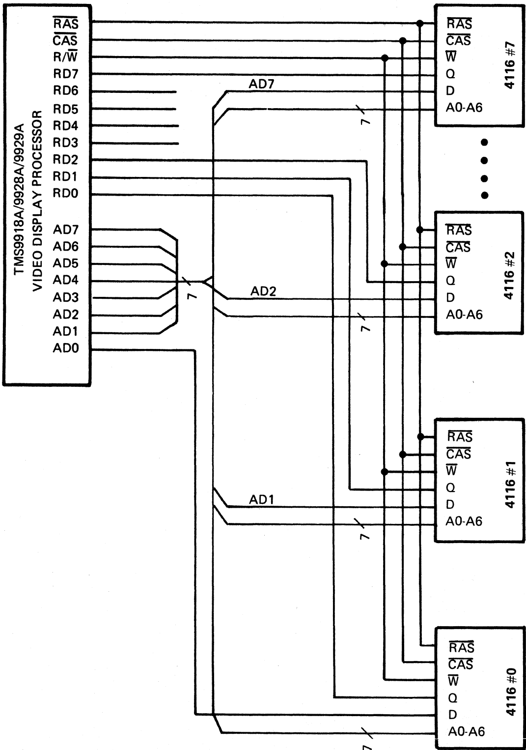
FIGURE 3-1 — VRAM INTERFACE
