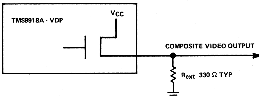
FIGURE 3-3 — COMPOSITE VIDEO PULL-DOWN CIRCUIT
