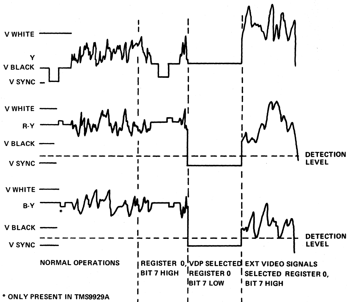
FIGURE 2-6 — TMS9928A/9929A SIGNAL WAVEFORMS FOR MULTIPLE VDP OPERATION
