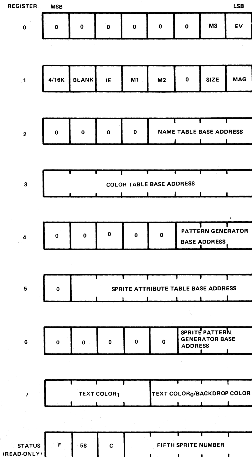
FIGURE 2-3 — VDP REGISTERS
