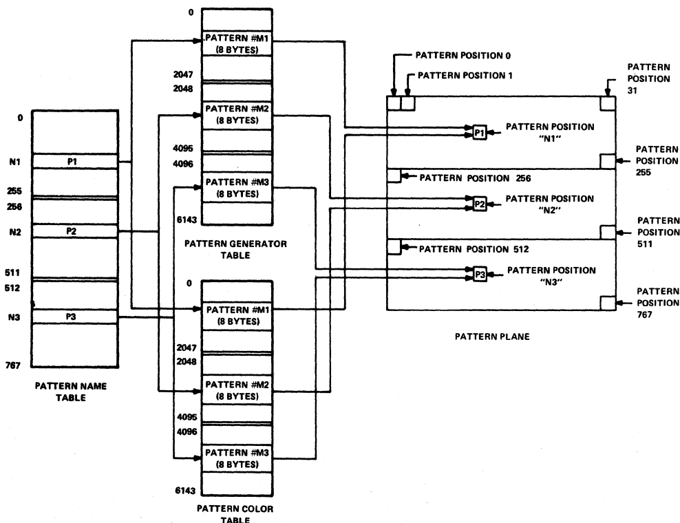
FIGURE 2-12 — GRAPHICS II MODE MAPPING
