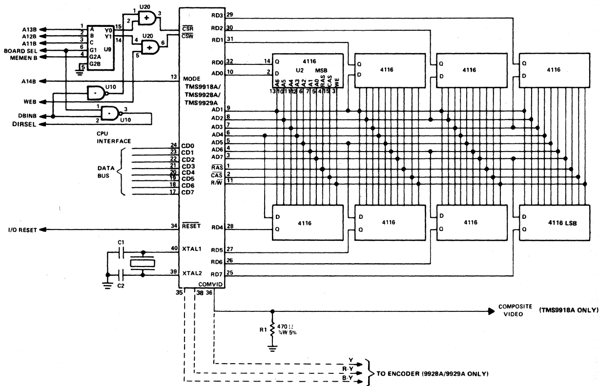
FIGURE 4-2 — TMS9918A/9928A/9929A INTERFACE
