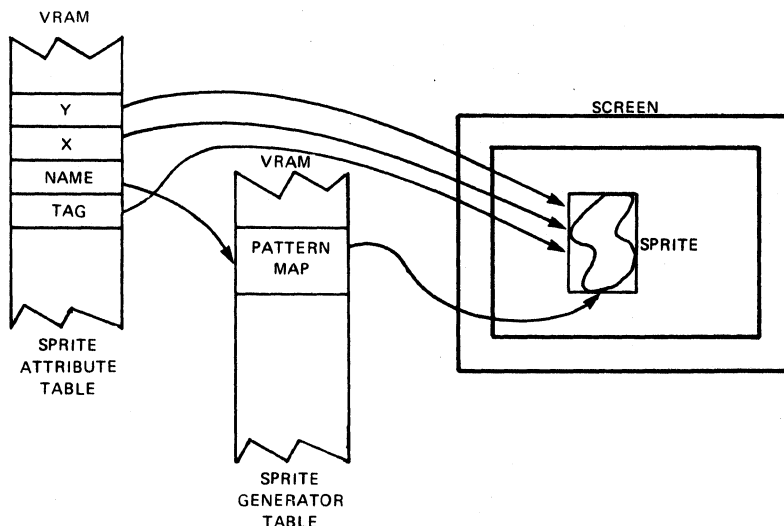
FIGURE 2-20 — SPRITE MAPPING
