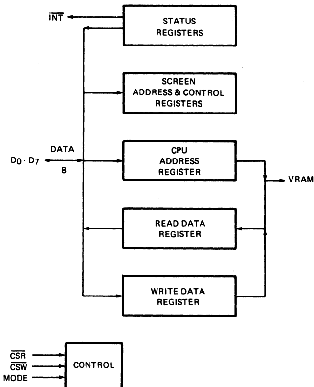
FIGURE 2-2 — VDP TO CPU INTERFACE
