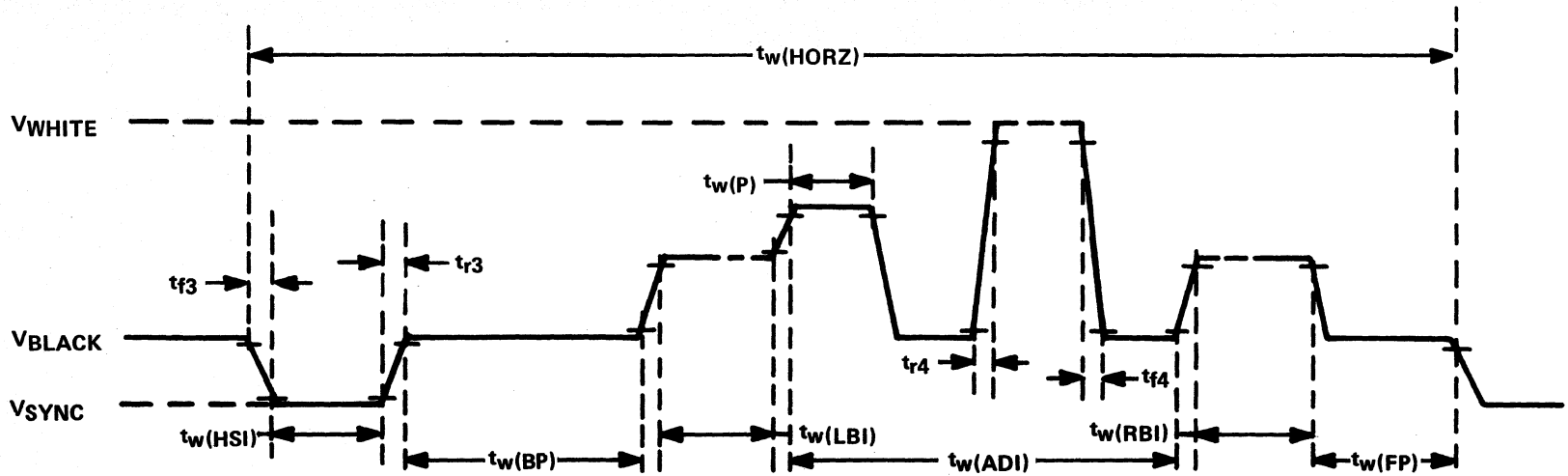
FIGURE 5-10 — TMS9928A/9929A Y HORIZONTAL TIMING
