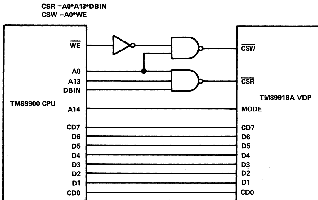
FIGURE 4-1 — MINIMUM SYSTEM INTERFACE TO TMS9900
