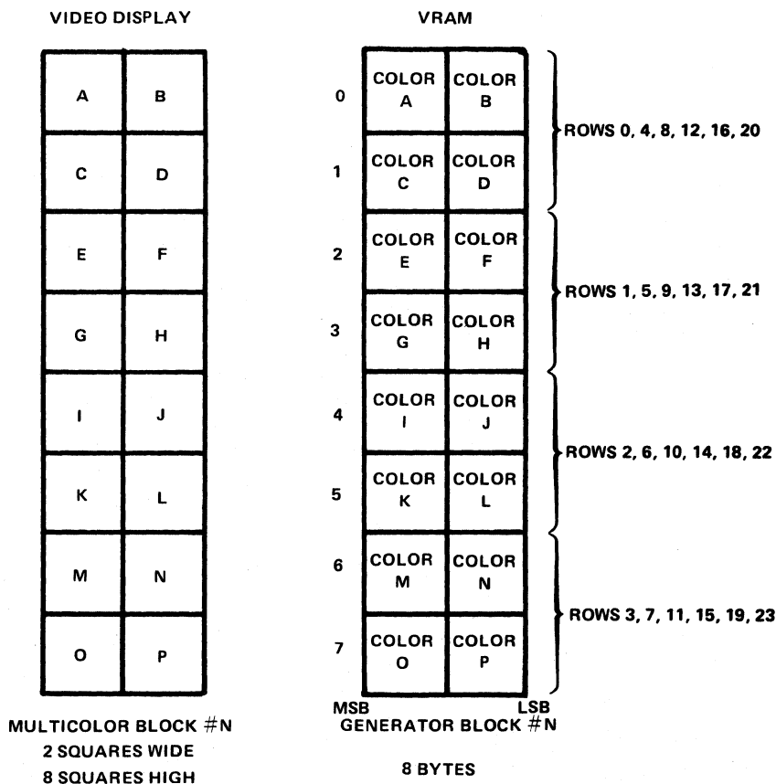
FIGURE 2-15 — MULTICOLOR BLOCK DISPLAY
