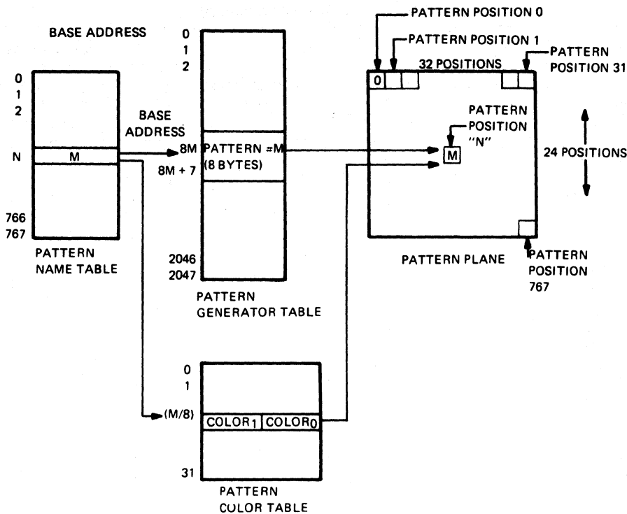
FIGURE 2-10 — GRAPHICS I MODE MAPPING
