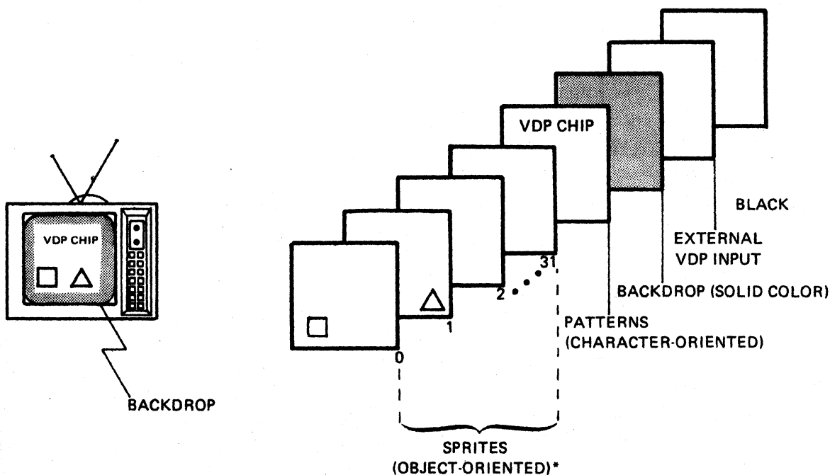
FIGURE 2-4 — VDP DISPLAY PLANES (DEFINITION)
