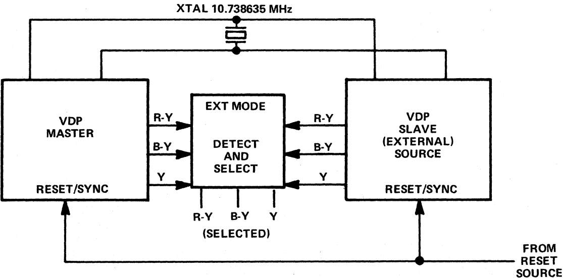
FIGURE 3-6 — CASCADING TWO TMS9918A/9929A VDPs
