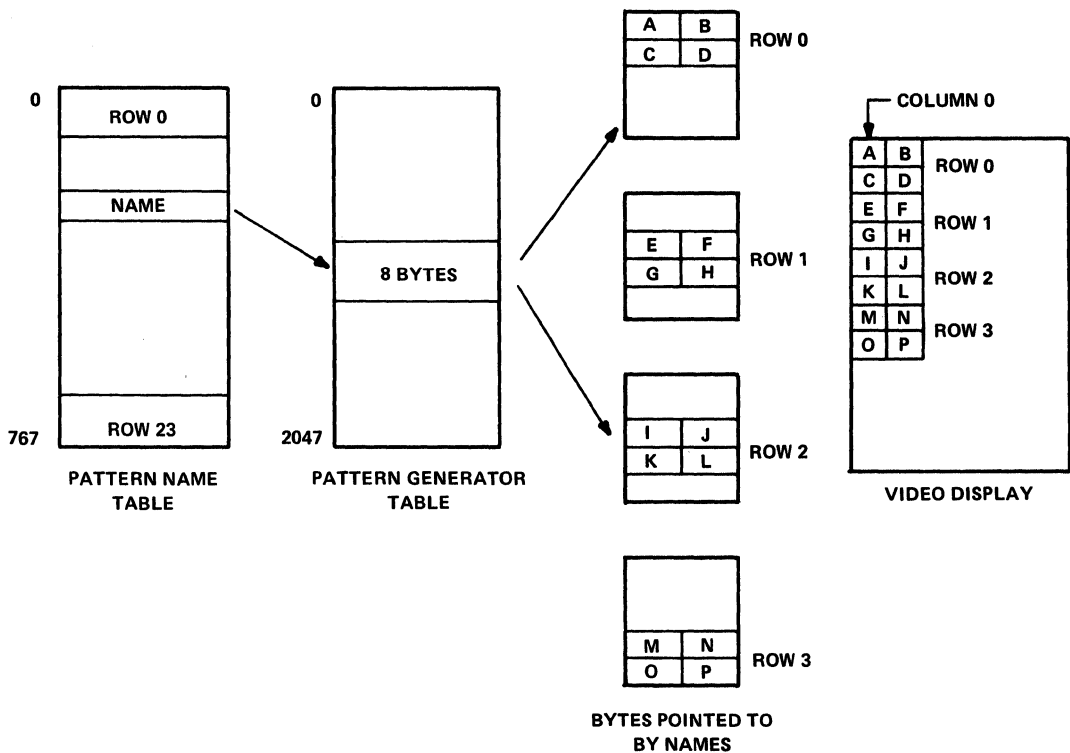
FIGURE 2-16 — MULTICOLOR MODE MAPPING
