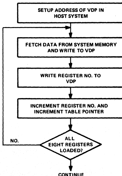
FIGURE 4-6 — VDP REGISTER INITIALIZATION PROCEDURE
