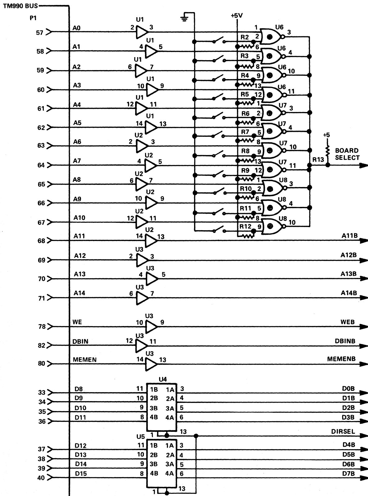
FIGURE 4-3 — TM990 (TMS9918A/9928A/9929A) DEMO BOARD
