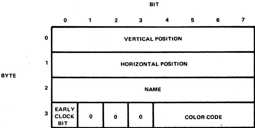
FIGURE 2-19 — SPRITE ATTRIBUTE TABLE ENTRY
