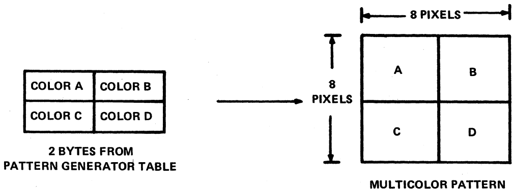
FIGURE 2-14 — MULTICOLOR LIST MAPPING
