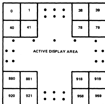
FIGURE 2-17 — TEXT MODE NAME TABLE PATTERN POSITIONS
