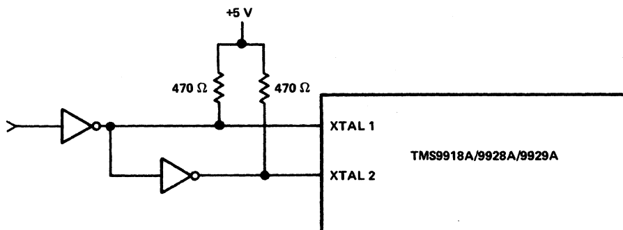
FIGURE 4-5 — EXTERNAL FREQUENCY SOURCE
