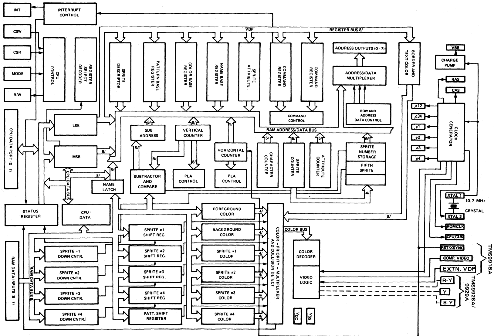
FIGURE 2-1 - VDP BLOCK DIAGRAM
